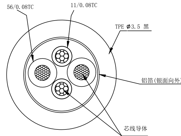
CABLE SPEC
